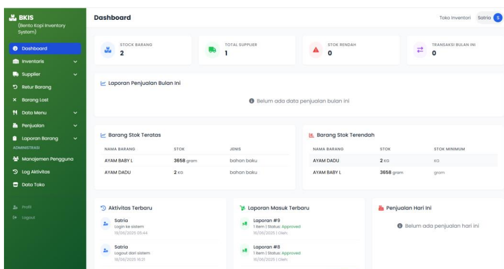
Figure 11. Dashboard Display
