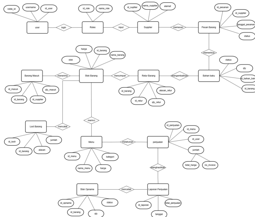
Figure 7. ERD
